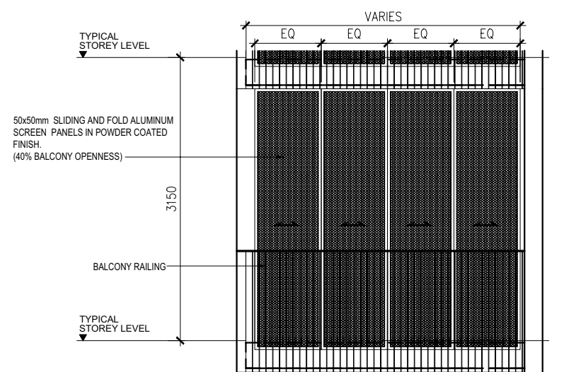
BALCONY / PES SCREEN - FRONT ELEVATION (External View)
